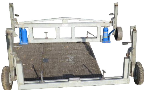
Hydraulic Pit Lid Lifter
